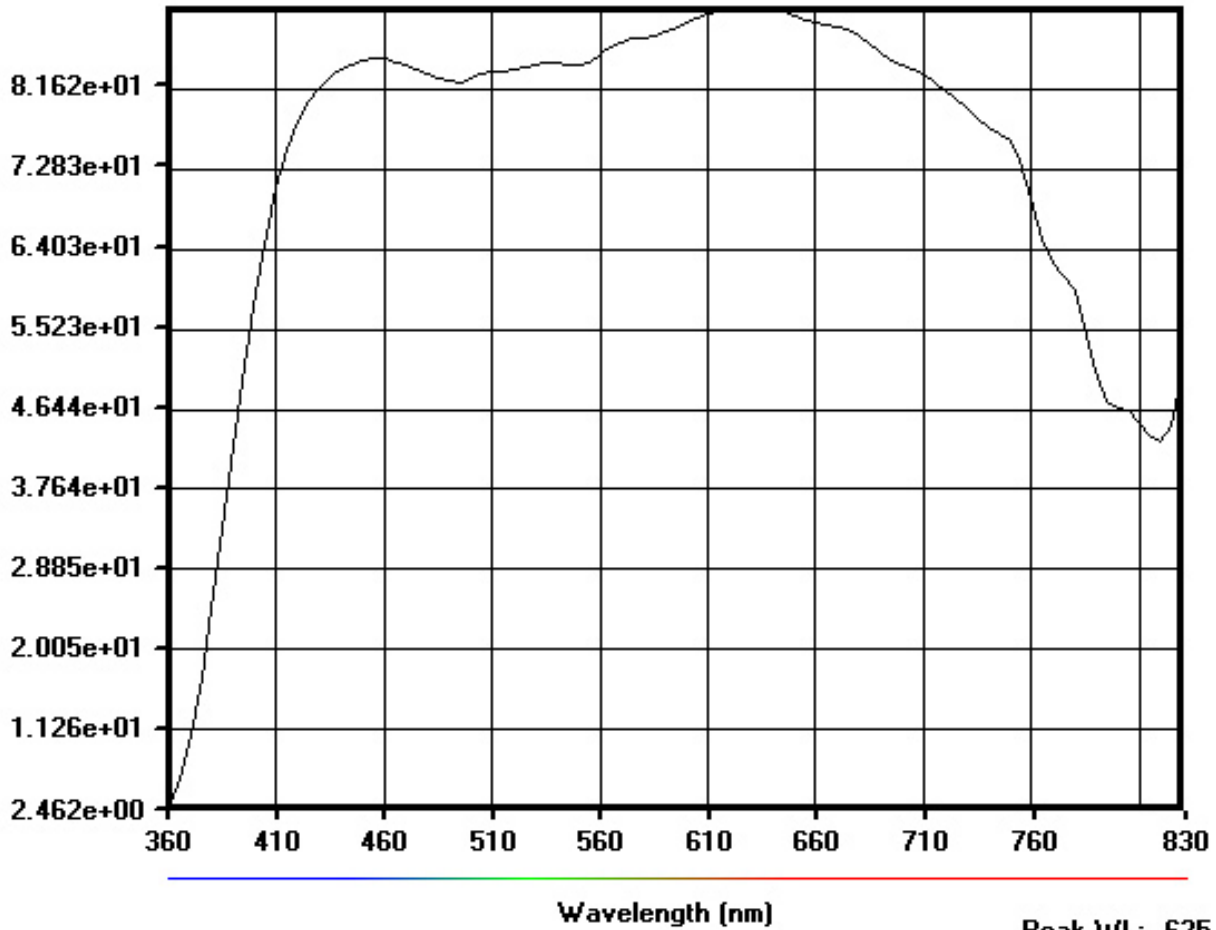
CARSON XM HD 8X42MM RIGHT TRANSMITTANCE FINAL 01/06/06
