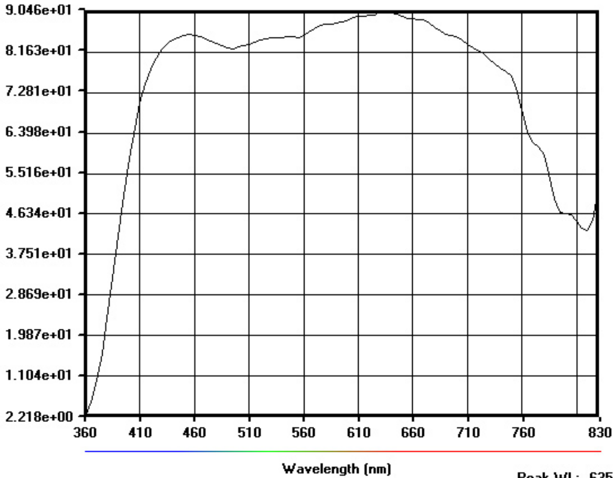
CARSON XM HD 8X42MM LEFT TRANSMITTANCE FINAL 01/06/06
